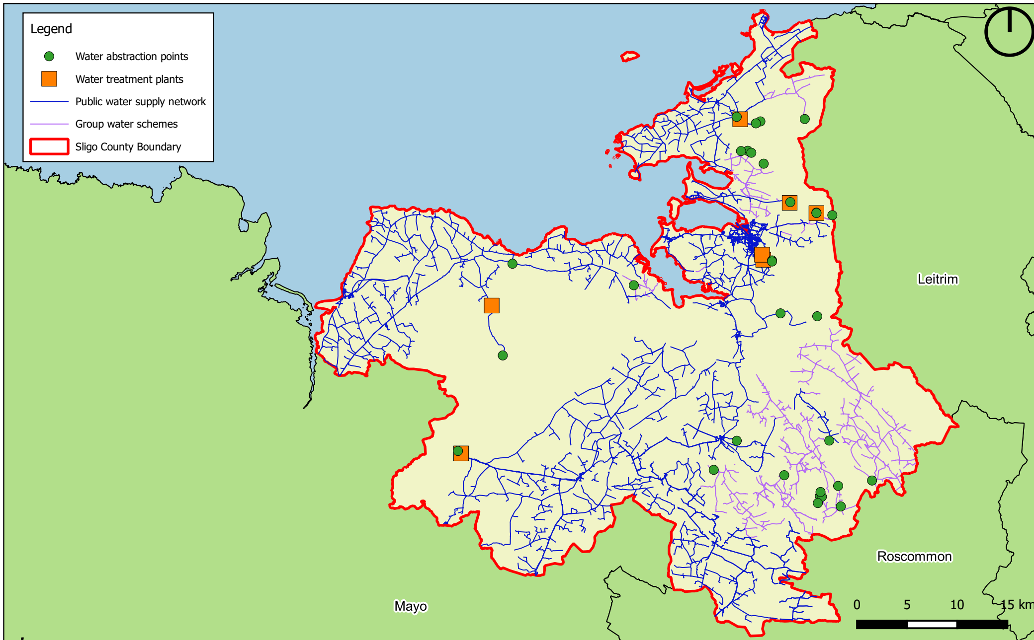
Map 30: Water abstraction points, treatment plants and water supply network
